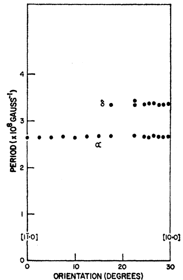
FIG. 3. Angular variation of the de Haas-van Alphen periods in zirconium in the (00\cdot1) plane. Data were taken at a temperature of \approx 1.1^\circ\text{K} .
